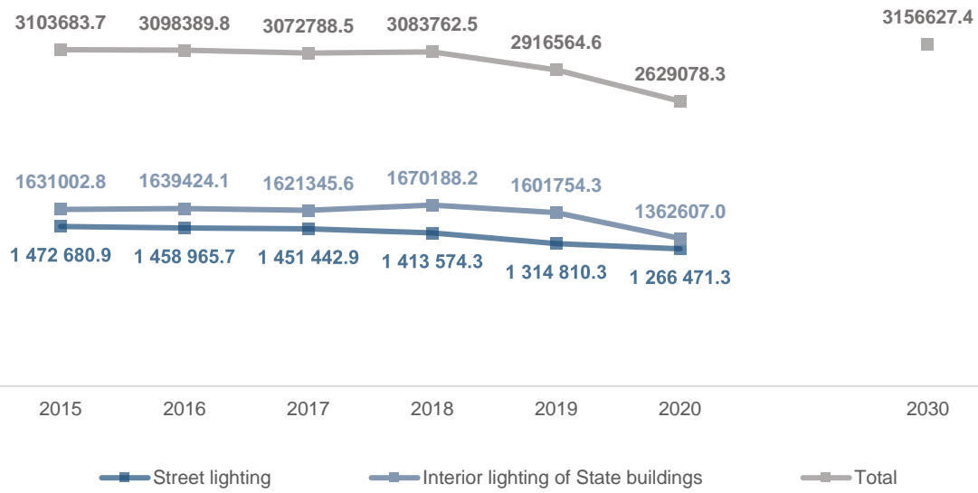
Electricity consumption for street lighting and interior lighting of State buildings (kWh) - Portugal
